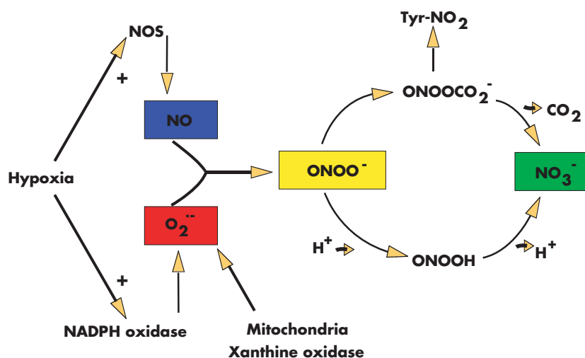
Figure 2 Simplified proposed model of NO reaction with superoxide ( O_2^- ). NO undergoes a direct bimolecular reaction with O_2^- yielding peroxynitrite ( ONOO^- ) at almost diffusion limited rates ( k=6.7 - 19 \times 10^9/M/s ). The rate constant is over 3.5 times faster than the dismutation of O_2^- by superoxide dismutases. By rapidly consuming superoxide, NO produces ONOO^-/ONOOH , a far less reactive oxidant than superoxide that can be further metabolised to innocuous products like NO_3^- . Tyr- NO_2 , nitrotyrosine.
