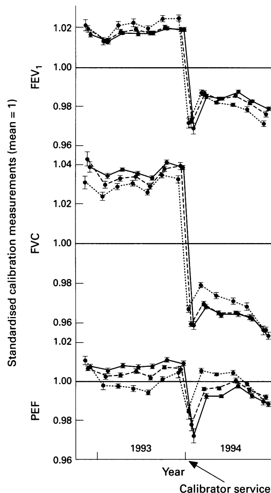
Figure 2 FEV 1 , FVC and PEF measurements obtained by calibrating 30 small turbine spirometers with a calibrator at three fixed inflation pressures: 0.2 bar (.....), 0.3 bar (---), and 0.4 bar(—). All measurements were divided by the overall mean of measurements at that particular inflation pressure, and each point represents the mean of a two month period. Bars indicate the standard error of the mean.
