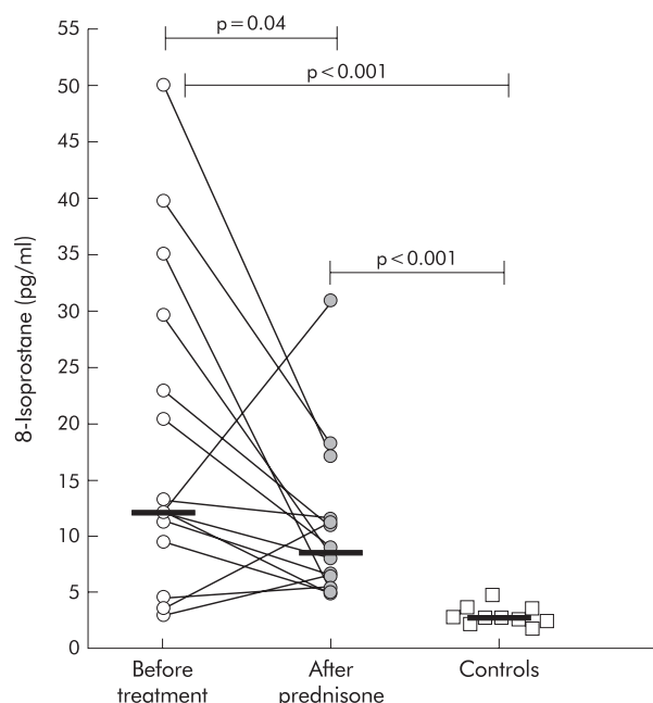
Figure 2 Exhaled breath condensate concentrations of 8-isoprostane in healthy controls and children with acute asthma before and after 5 days of treatment with prednisone. Individual and median values are shown.
